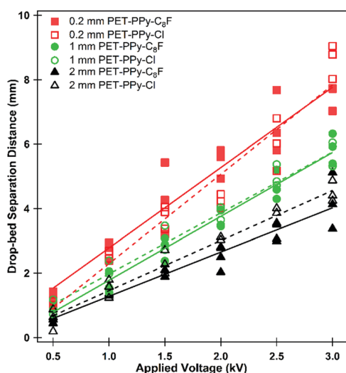
Fig. 6 Drop-bed separation distance at which particles began to be extracted from the particle bed for each studied applied potential as the particle bed approaches the 5 \mu\text{L} pendent water drop at 0.05 \text{mm s}^{-1} . Lines do not denote a physical relationship but are present to guide the eye.
